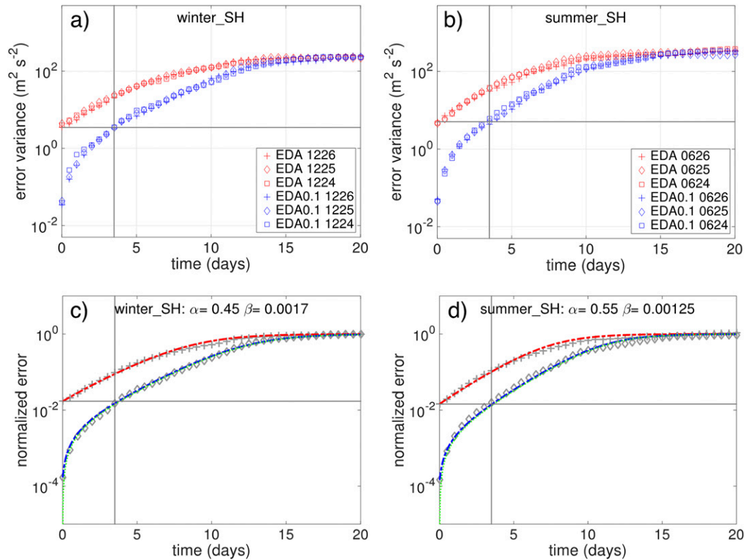
FIG. 4. As in Fig. 3, but for SH (40°–60°S).
