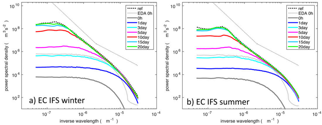
FIG. 6. Forecast error growth and saturation for different horizontal scales. Evolution of ensemble-mean error spectral kinetic energy (colored lines) averaged over NH midlatitudes ( 40^{\circ} – 60^{\circ} N) for three 9-km, 10-member ECMWF IFS global ensemble simulations with minute (1%) initial-condition errors (solid gray lines) initialized on 3 consecutive days for (a) the winter period and (b) the summer period. The reference background kinetic energy spectra are derived from the respective 20-day mean spectra of the control forecast (dark dotted line). The corresponding initial spread of the EDA ensemble with realistic analysis uncertainties are shown for comparison (light-gray dotted lines). The two straight dotted line segments denote the spectral slopes of -3 and -5/3 .
