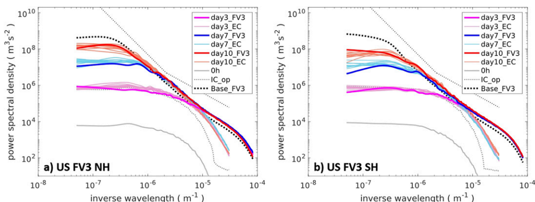
FIG. 8. Sensitivity of error growth and saturation with the 3-km FV3 model. Evolution of perturbation spectral kinetic energy between two forecasts (one initialized with the control EDA analysis and the other perturbed with the same initial perturbations as in EDA0.1 ensemble member 1 performed with the 3-km U.S. FV3 model for (a) NH and (b) SH. Computational costs permit us to run only one pair of 10-day simulations starting at 0000 UTC 24 Dec 2015 for the winter event. Thin lines show results for EC model calculated based on the differences between 10 perturbed EDA0.1 members and the control run. The FV3 results lie well within the 10 ensembles produced by the EC model. Note at small scales, different with the perturbation kinetic energy spectra in Fig. 6, the difference spectral kinetic energy has a saturation level that is twice the background spectrum.
