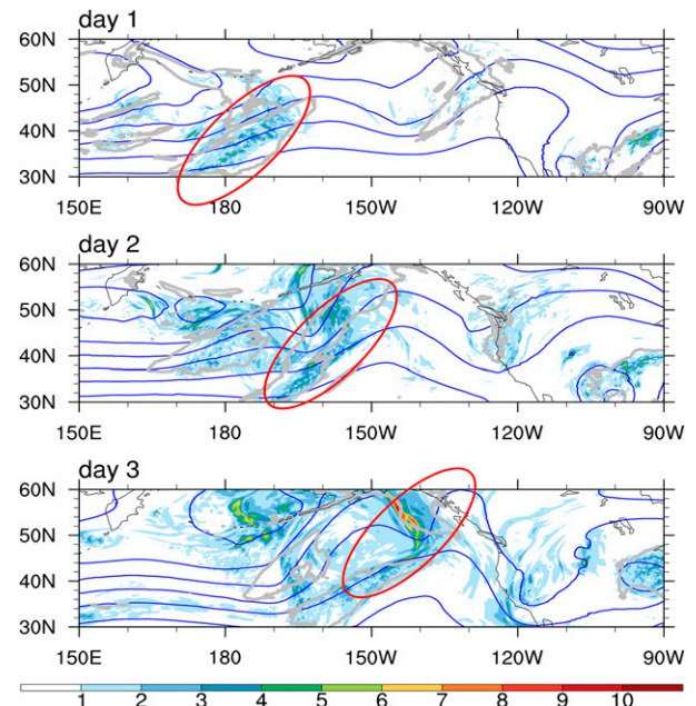
FIG. 9. Evolution of the ensemble spread of 500-hPa meridional winds (color-shaded) for the first 3 days in EDA0.1 integrated from 0000 UTC 26 Dec 2015. Blue contours are the 500-hPa geopotential heights, and gray contours indicate the regions with 12-h precipitation greater than 0.1 mm. Red circles imply the movement of the developing low pressure synoptic storms.
