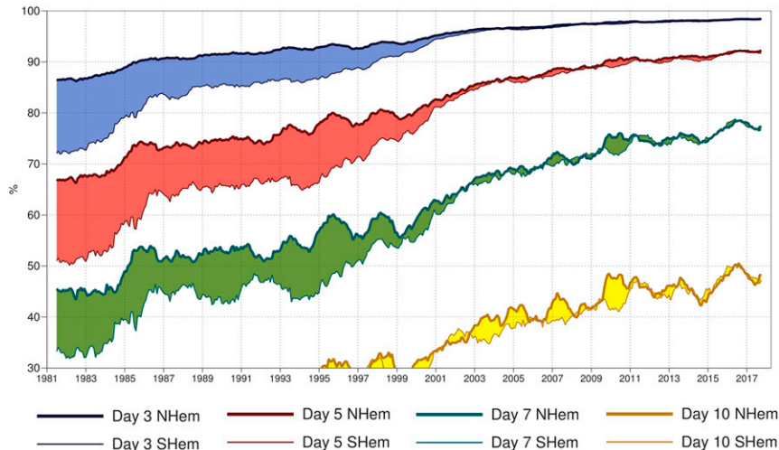
FIG. 1. Annual evolution the ECMWF NWP deterministic control forecast performance in terms of anomaly correlation of 500-hPa-height predictions. Shading indicates the different forecast skill between NH and SH, which has almost disappeared in recent years. This plot is directly adapted from ECMWF official website ( https://www.ecmwf.int/en/forecasts/charts/catalogue/plwww_m_hr_ccaf_adrian_ts ).
