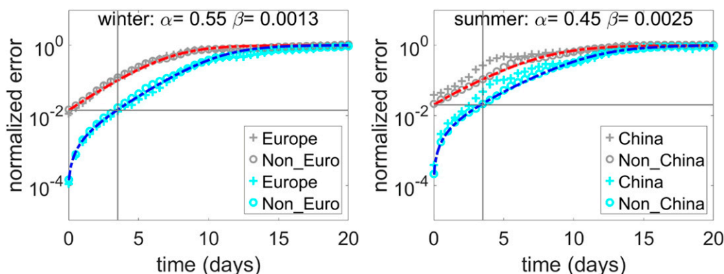
FIG. 11. As in Figs. 3c and 3d, but separating the error statistics in the hazardous-event region vs the rest of the midlatitudes. Red and blue curves are the same fitted curve as in Fig. 3, implying the global averaged results. The plus signs represent the hazardous-event region ( 60^\circ -longitude width), and the circles represent the nonhazardous-event region ( 300^\circ -longitude width).
