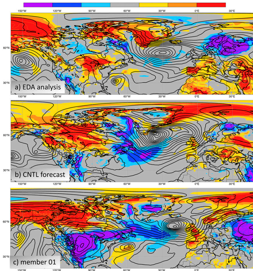
FIG. 2. Sample 15-day numerical weather predictions vs observations. The 2-m surface temperature anomalies (color shading) and the sea level pressure (contoured every 4 hPa) and valid at 0000 UTC 8 Jan 2016 for (a) the ECMWF observational analysis, (b) the 9-km IFS 15-day-lead-time control forecast initialized at 0000 UTC 24 Dec 2015 with the unperturbed EDA analysis, and (c) 15-day forecast from a member of the ensemble (EDA0.1) perturbed with 10% of the EDA ensemble perturbations that the current level of uncertainty in the EDA analysis. The temperature anomalies are calculated from a climatology based on a 20-yr, 10-member ensemble reforecast dataset using the same model with a 15-day lead time.
