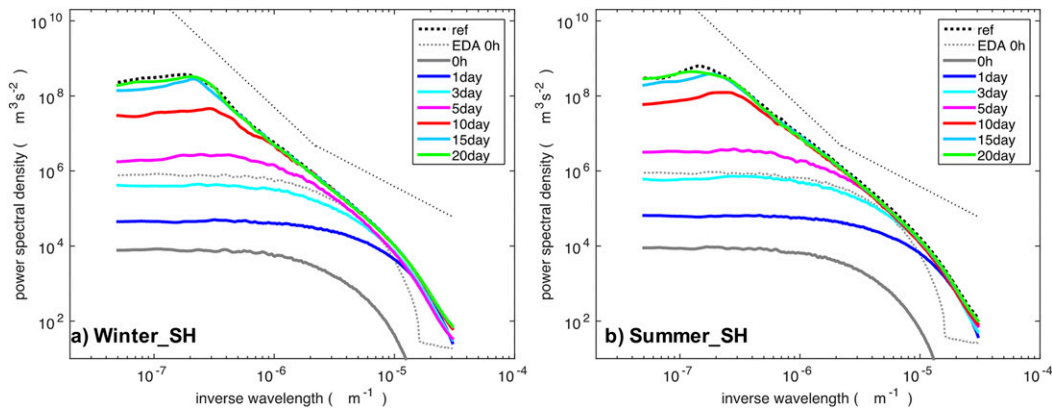
FIG. 7. As in Fig. 6, but for SH ( 40^{\circ} – 60^{\circ} S).
