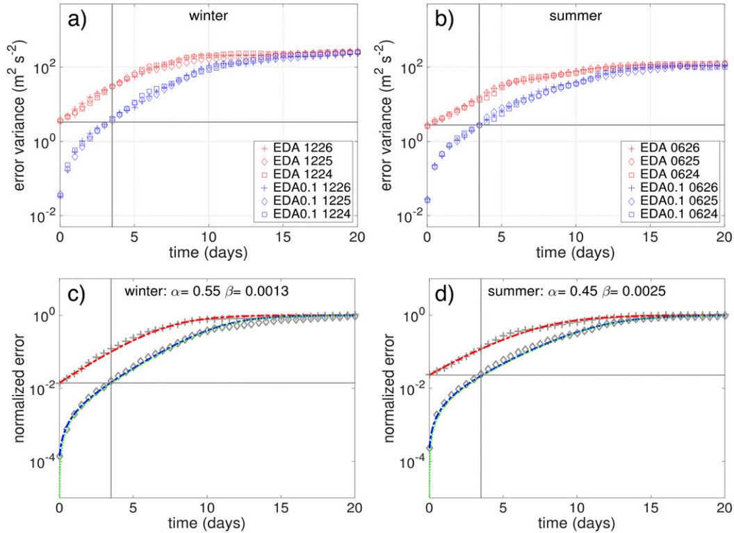
FIG. 3. (top) Evolution of forecast uncertainty growth in terms of ensemble variance of 500-hPa wind energy averaged over the NH midlatitudes (40°–60°N) for three ensemble simulations with current-day realistic initial-condition uncertainties (red symbols) and the corresponding ensembles with minute (1%) initial-condition errors (blue symbols) initialized on (a) 3 consecutive days for the winter (24–26 Dec 2015) and (b) 3 consecutive days in the summer (24–26 Jun 2016). (bottom) Evolution of normalized error variances (gray symbols) averaged for the (c) winter and (d) summer cases, as well as the fitted error growth curves (red for EDA, blue for EDA0.1) from Eq. (1). The units for \alpha and \beta are \text{day}^{-1} . Green lines in (c) and (d) show the error growth curve according to the fitted Eq. (1) if the initial-condition error is further reduced to 1 \times 10^{-10} . Note the log scale of the perturbation energy.
