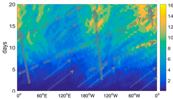
FIG. 10. Longitude–time Hovmöller diagram for the mean ensemble spread in terms of root-mean-square difference of kinetic energy ( \text{m s}^{-1} ) derived from the 9-km, 20-day, 10-member ECMWF IFS global ensemble initialized at 0000 UTC 24 Dec 2015 as a demonstration of different modes of error propagation that lead to the error saturation and intrinsic predictability limits (see text for details).
